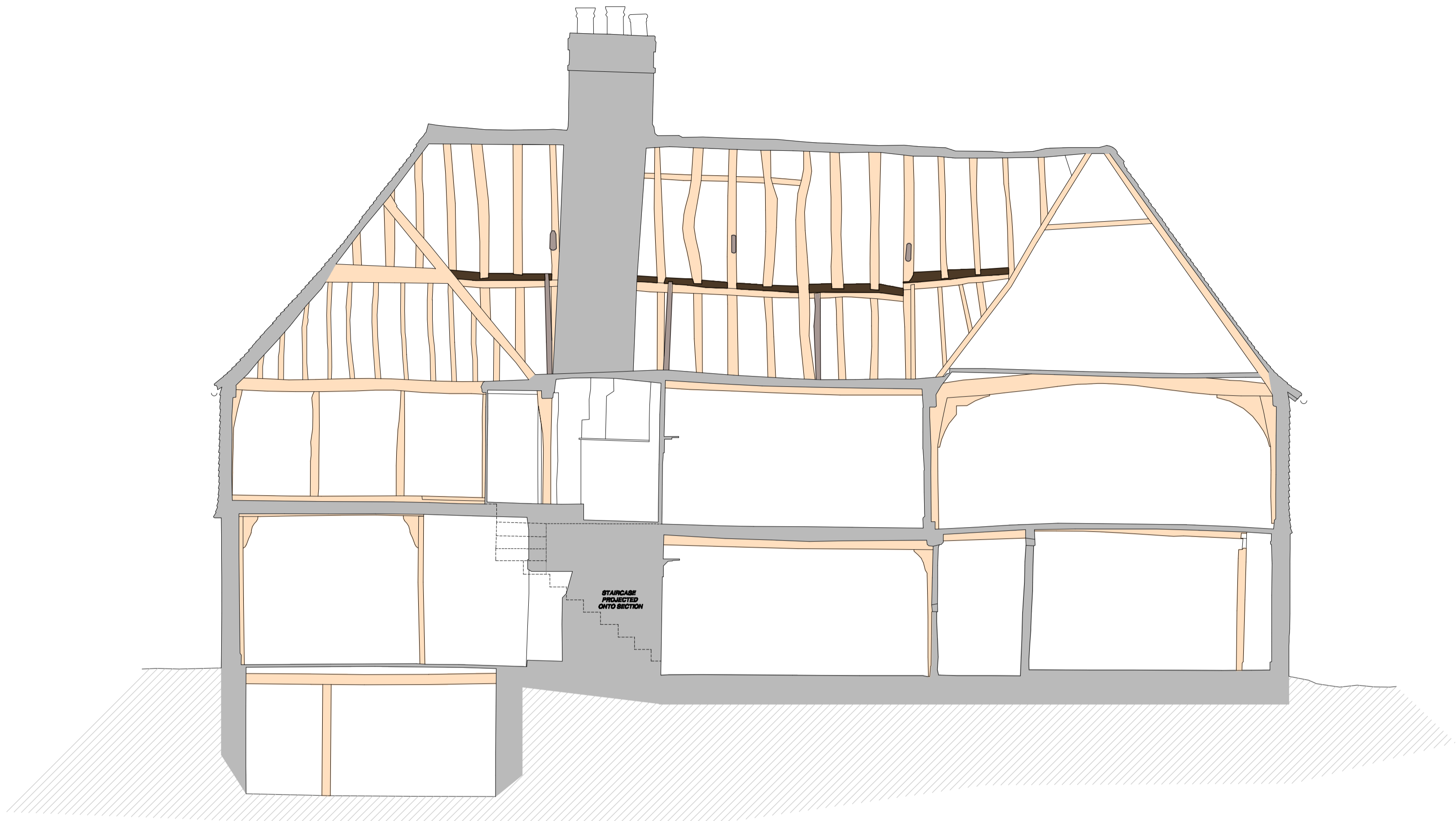
SECTION A-A ROOF FRAME DETAILS PROJECTED ONTO SECTION
